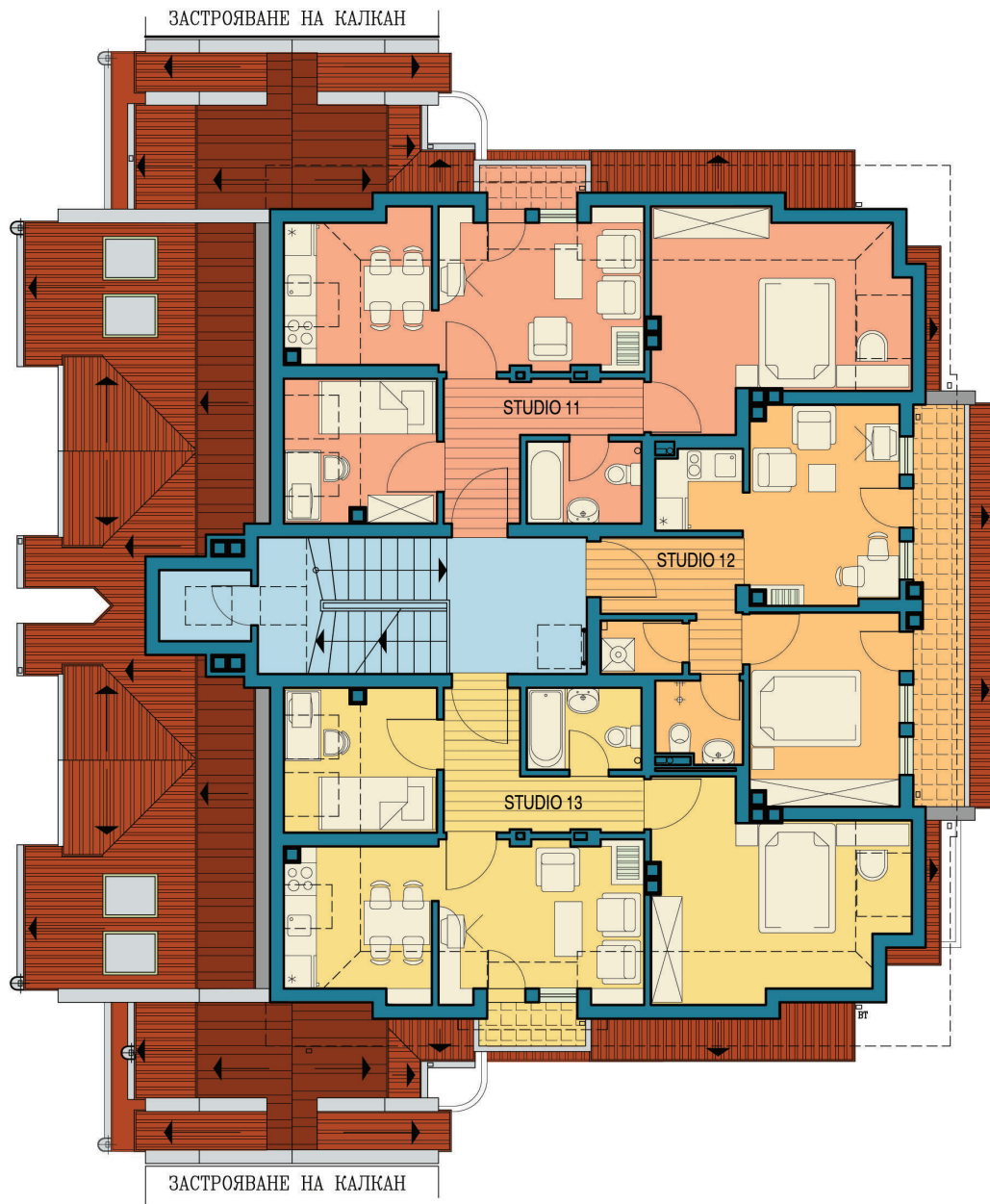
FOURTH FLOOR M 1:100
