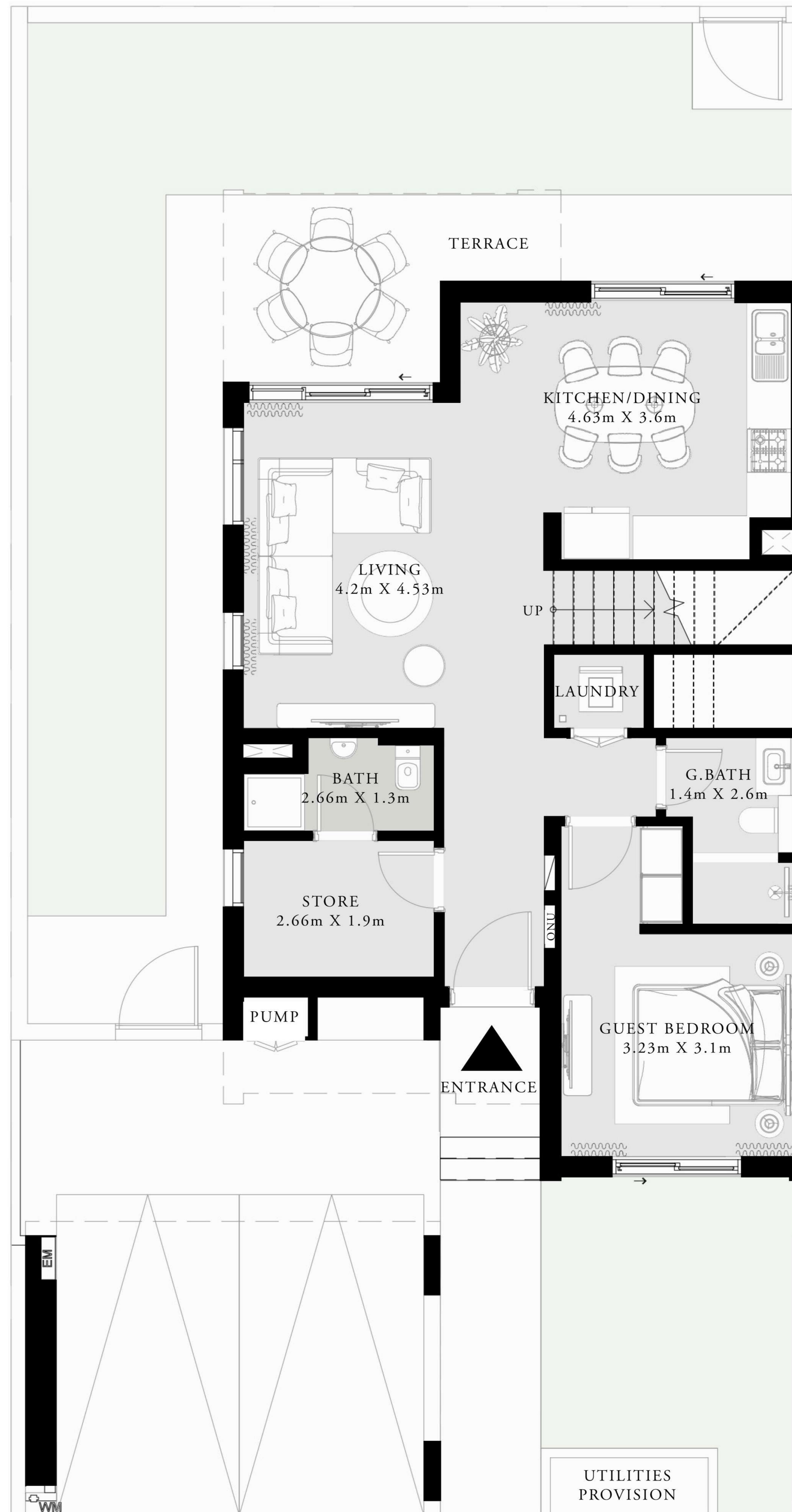
GROUND FLOOR
